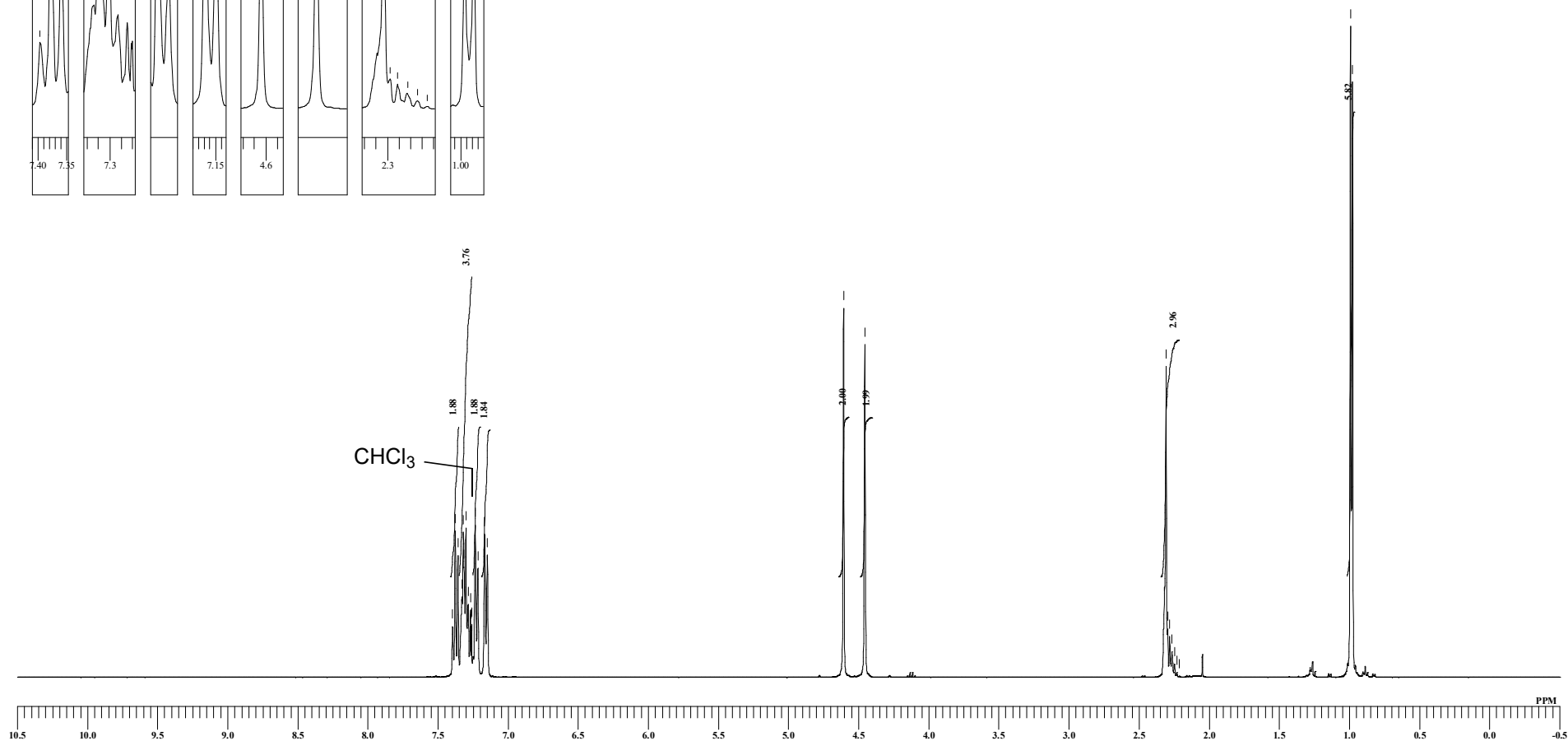
N,N -dibenzyl-3-methylbutanamide ( 2 ) 1 H NMR (500 MHz, CDCl 3 )
